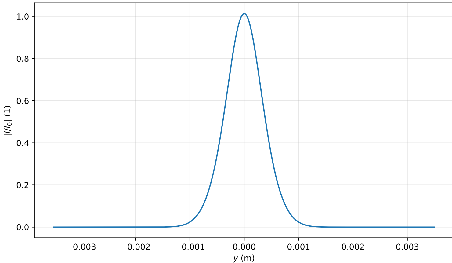
Intensity profile I(x=0, y, z=0.796)/I_0 , P_{in}=0.4P_{cr} , artificial time
